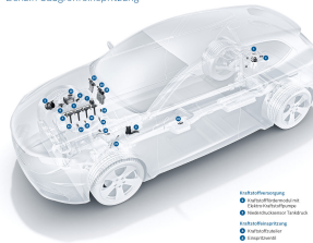
Benzin-Saugrohreinjection
