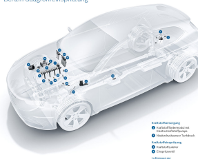
Benzin-Saugrohreinjection
